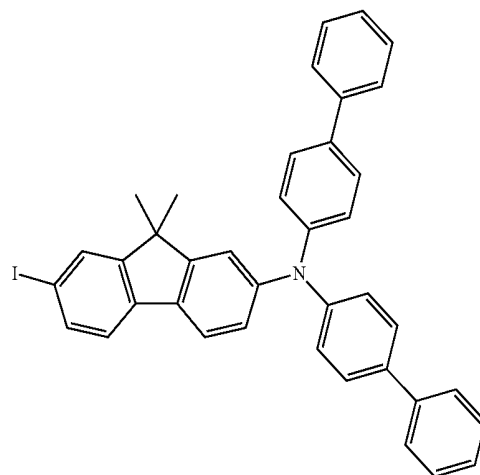
Intermediate 6
