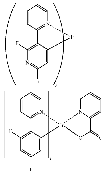
F 2 Irpic
