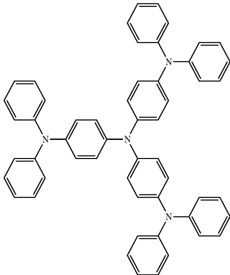
TDATA
